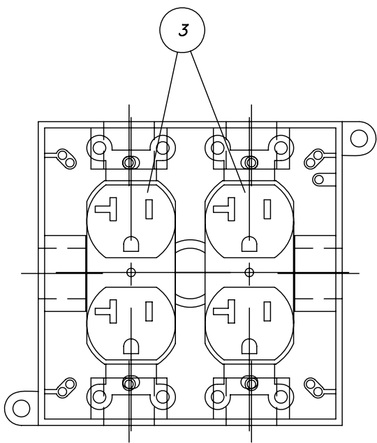
(COVER REMOVED FOR CLARITY)
