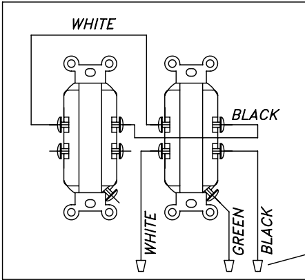
INSIDE BACK VIEW OF OUTLET BOX, REF
