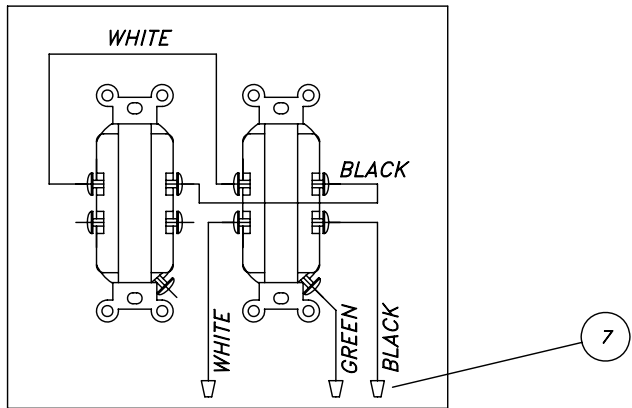
INSIDE BACK VIEW OF OUTLET BOX, REF
